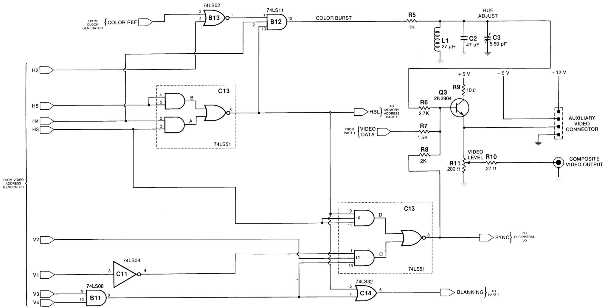
Fig. C-17. Video generator—part 2 (Rev. 0).
