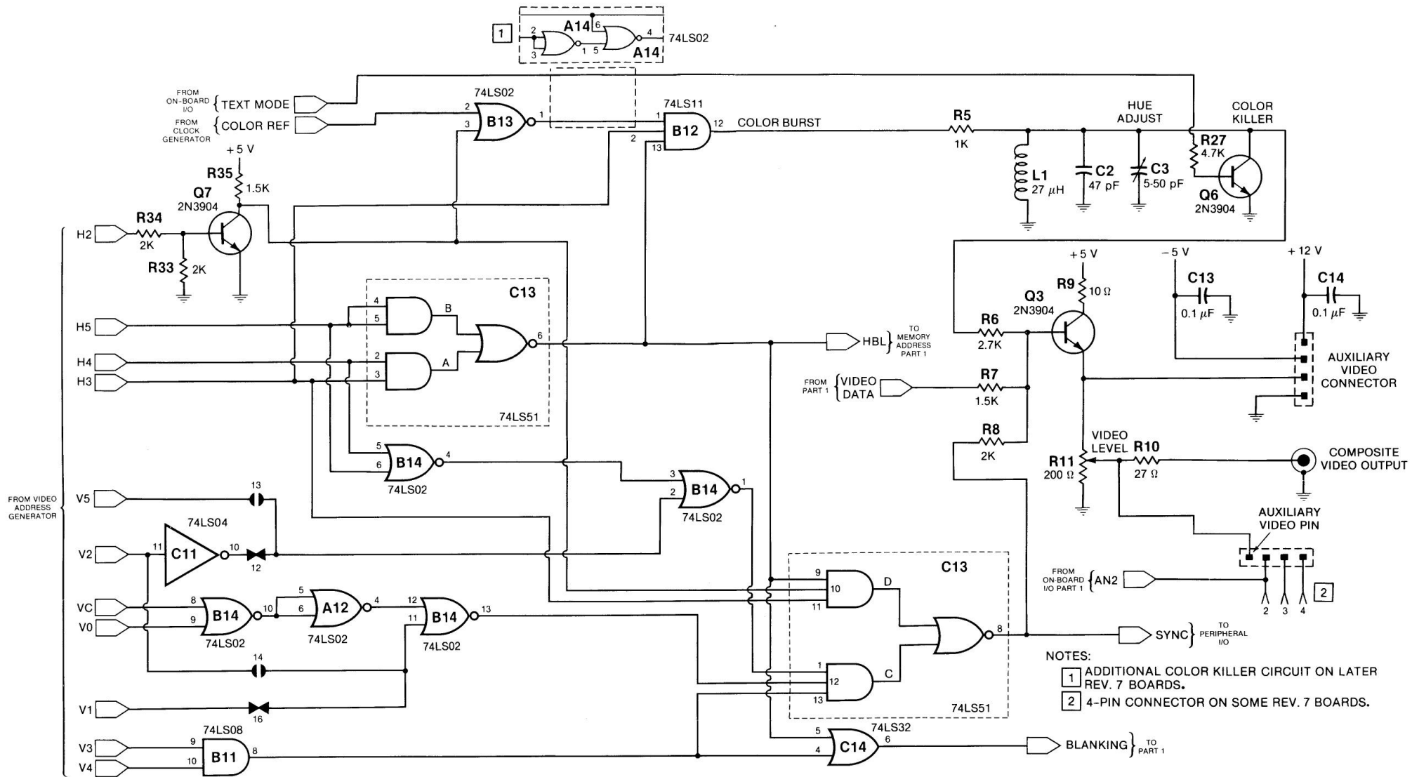
Fig. C-19. Video generator—part 2 (Rev. 7).
