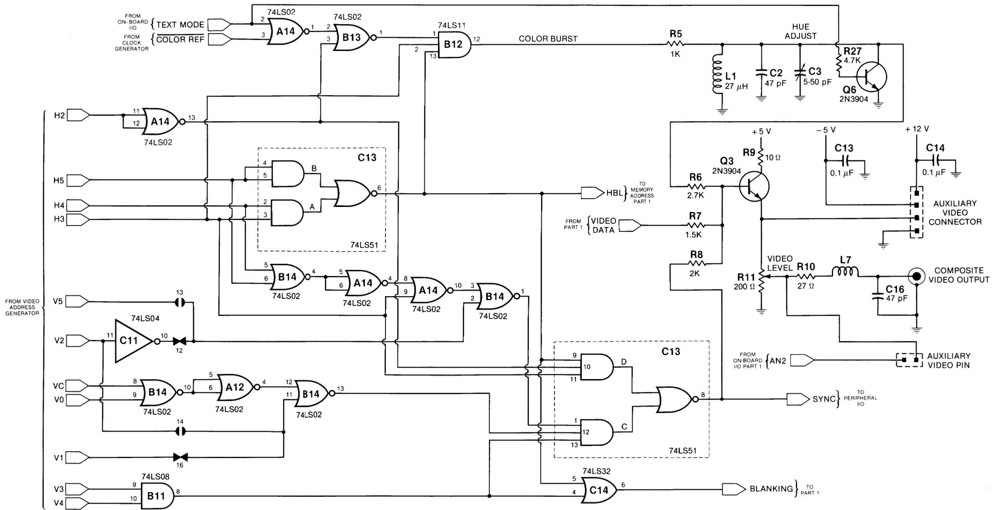
Fig. C-20. Video generator—part 2 (RFD).
