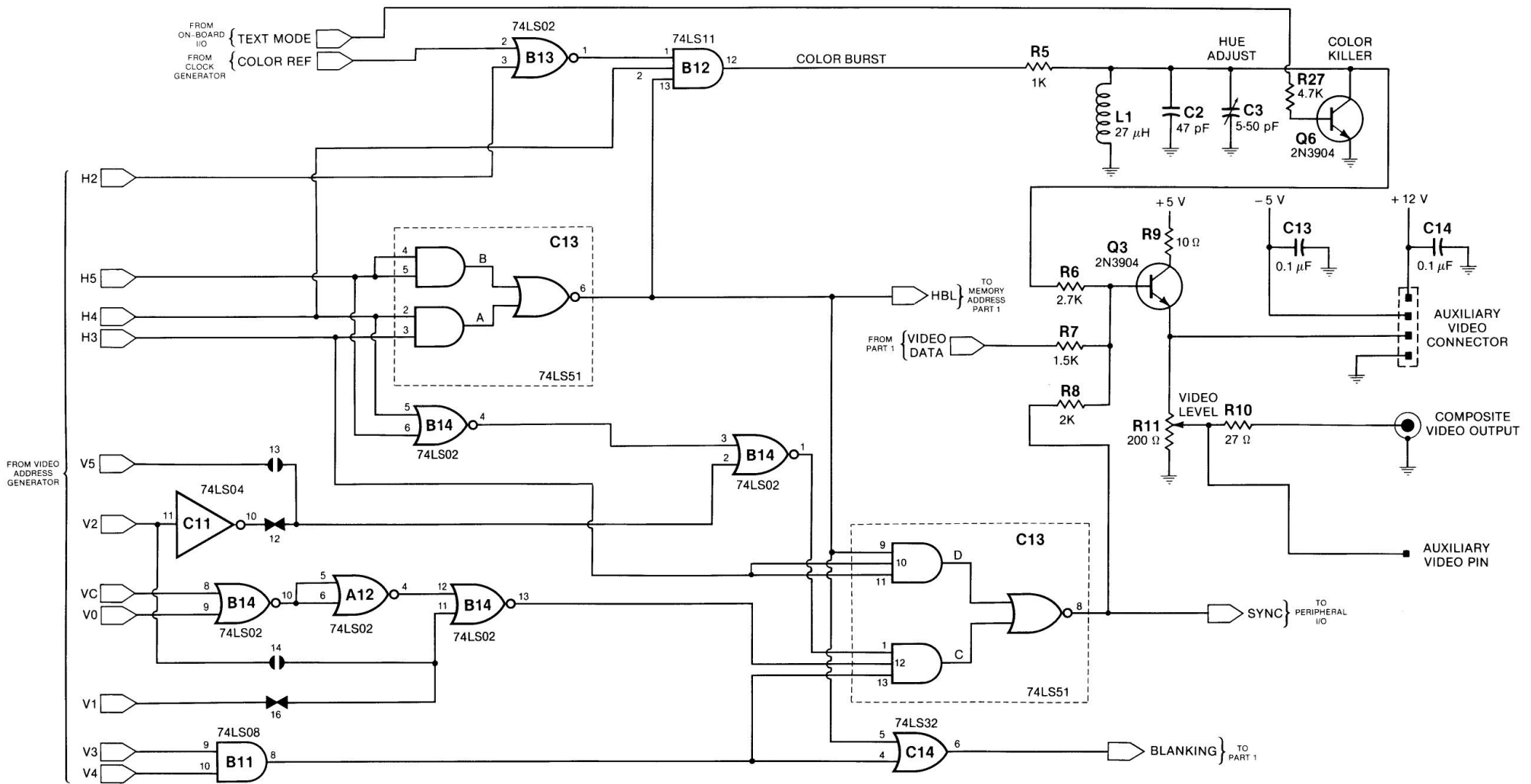
Fig. C-18. Video generator—part 2 (Rev. 1).
