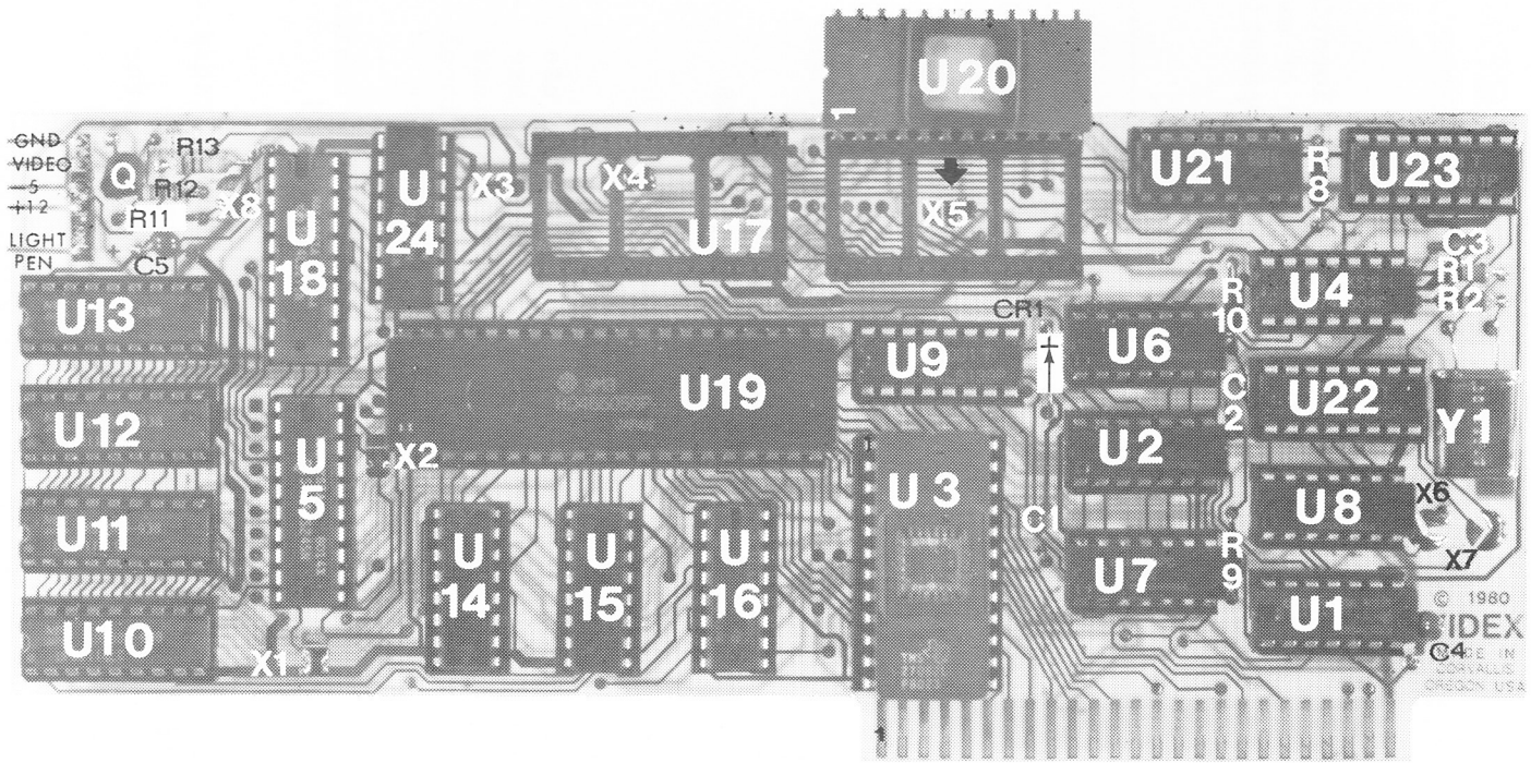
Figure 10: VIDEOTERM Board Photograph
