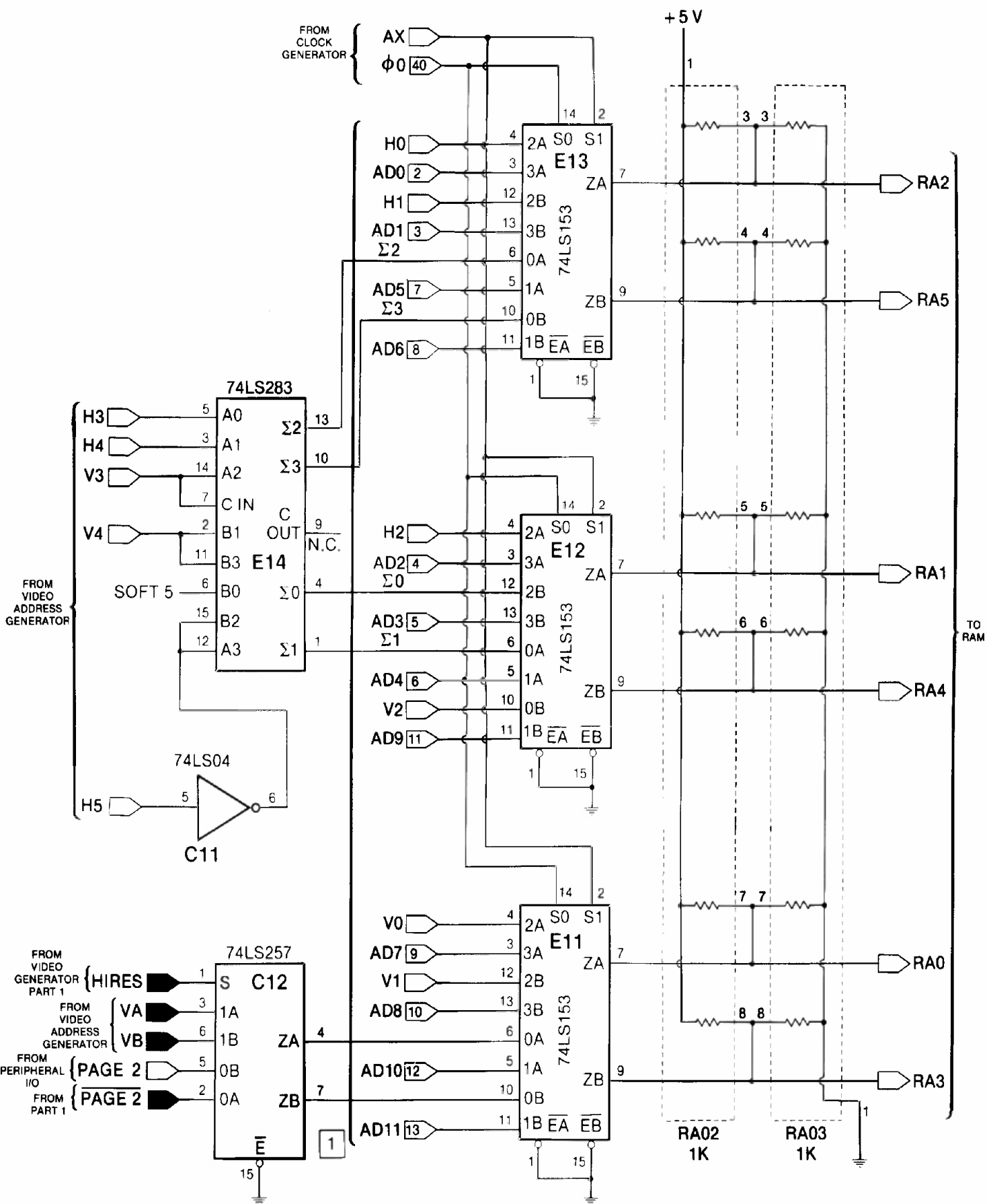
Fig. C-6. Memory address—part 2 (all revisions).
