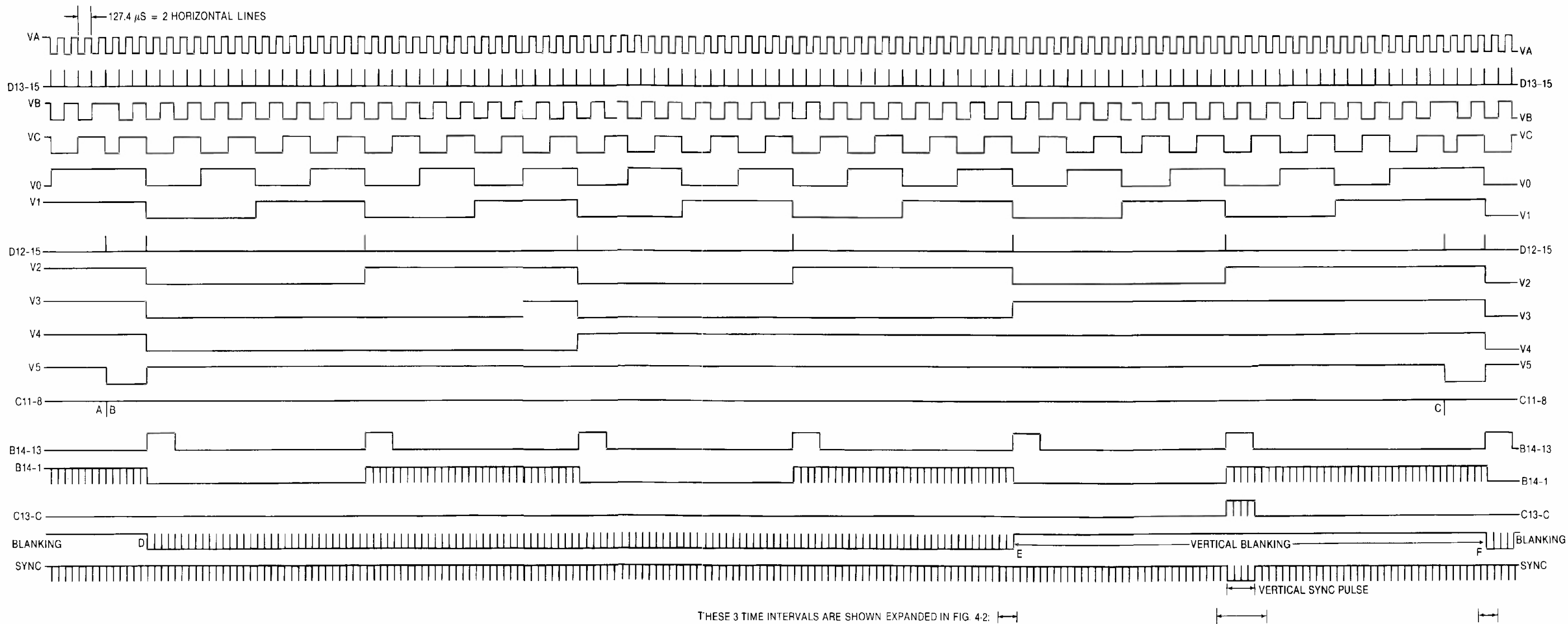
Fig. 4-1. Vertical timing
