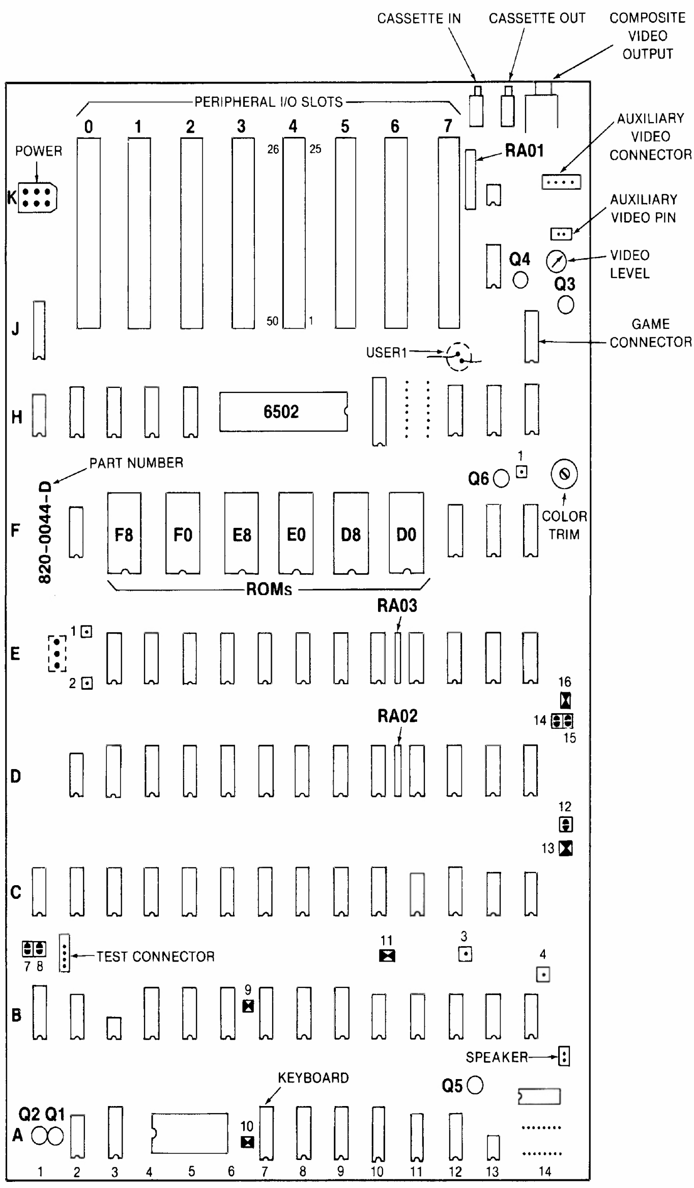
Fig. 1-1. Diagram of the Apple II RFI motherboard. (Courtesy Apple Computer Inc.)
