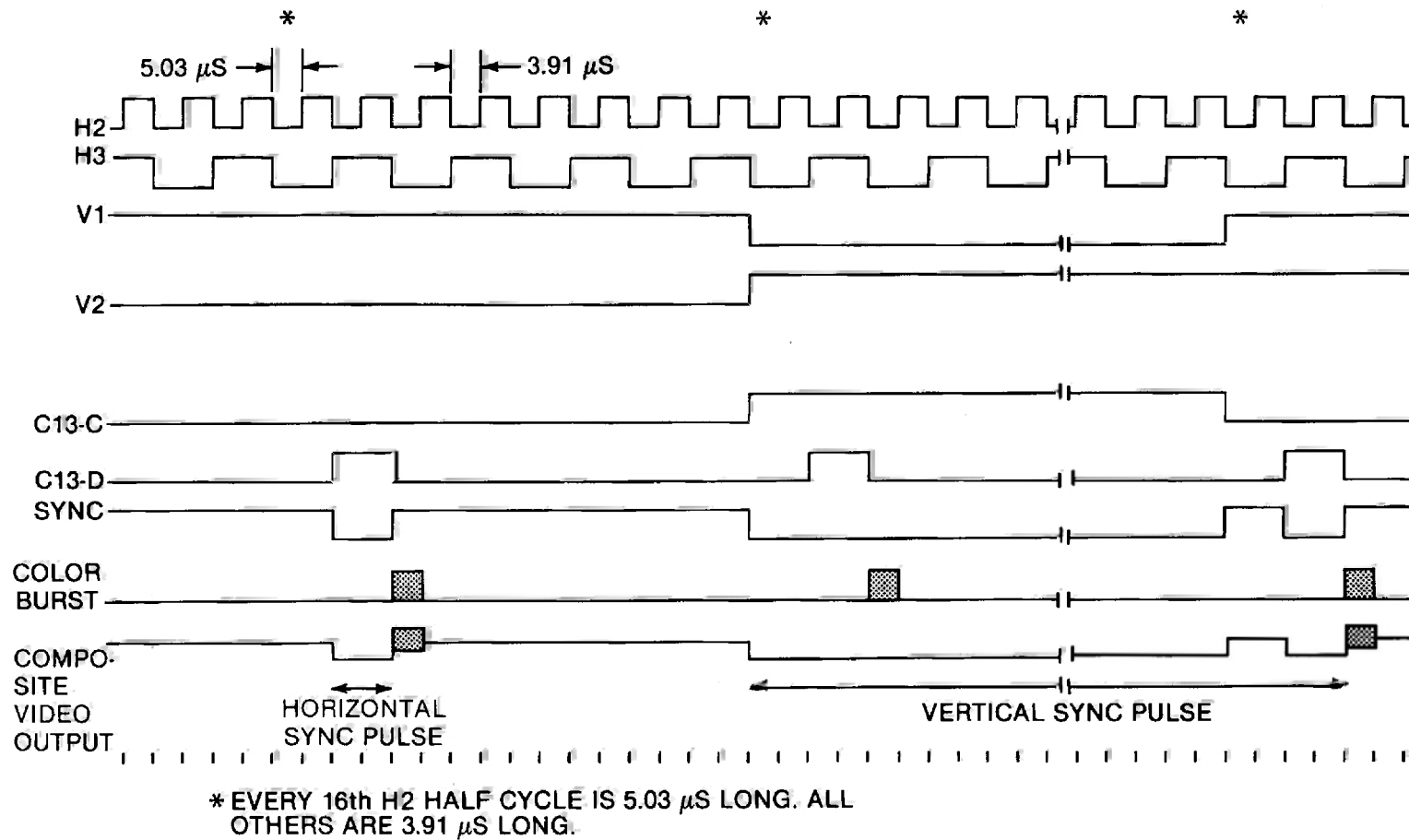
Fig. B-6. Vertical and horizontal sync—Rev. 0.
