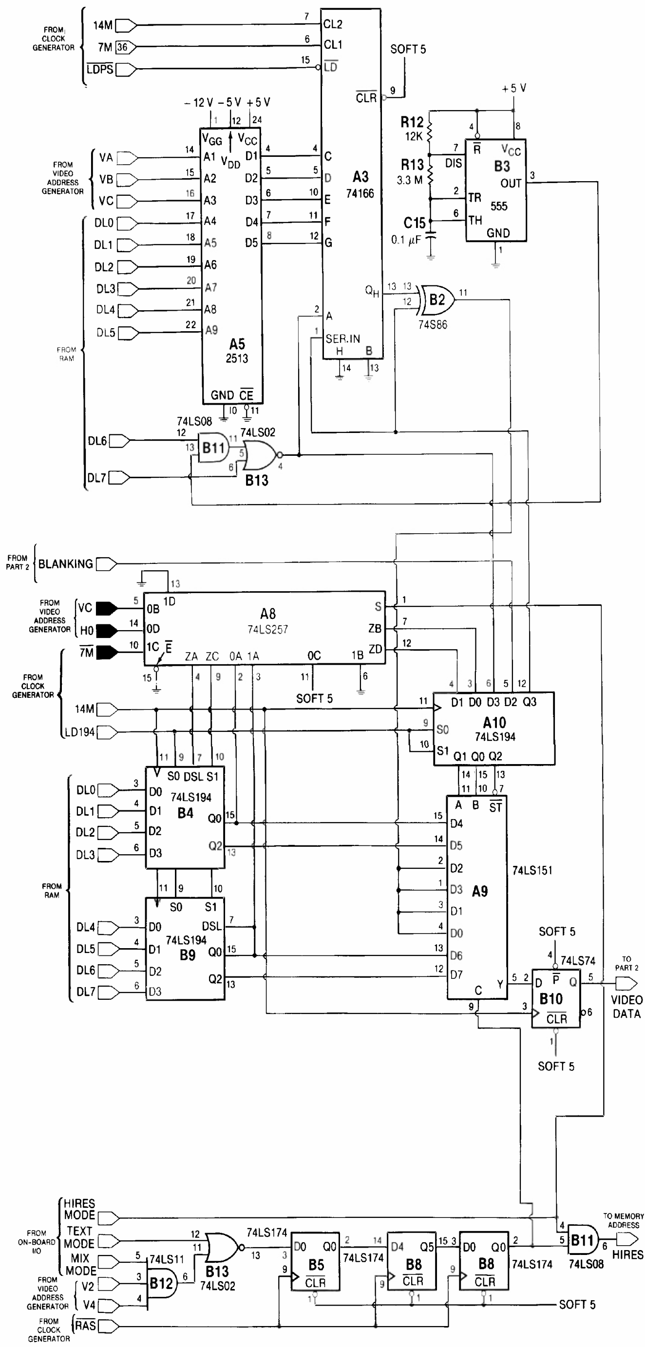
Fig. C-14. Video generator—part 1 (Rev. 0).
