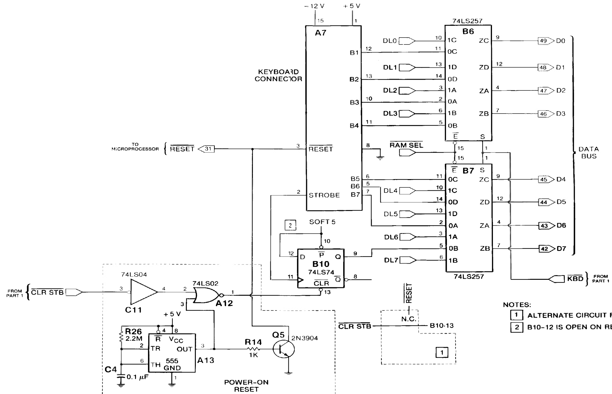
Fig. C-13. On-board I/O—part 2 (all revisions).
