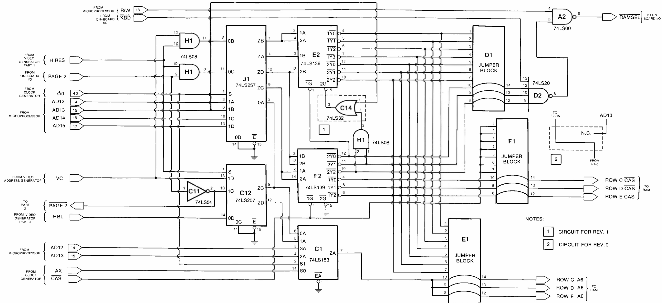
Fig. C-4. Memory address—part 1 (Rev. 0,1).
