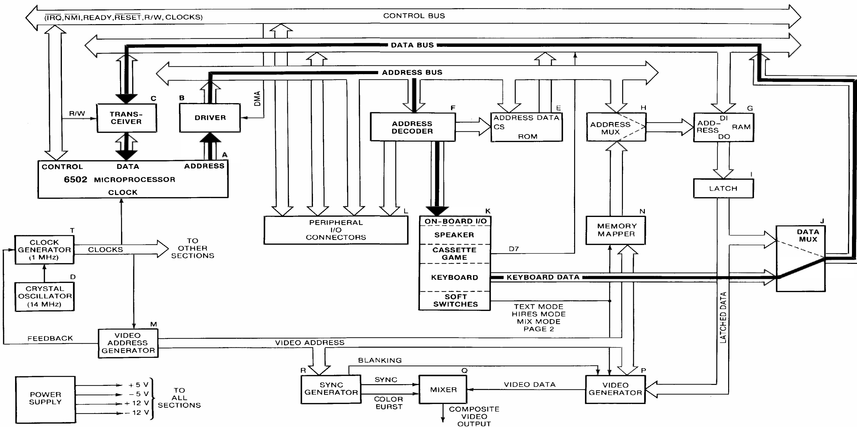
Fig. 2-5. Keyboard read-cycle path.
