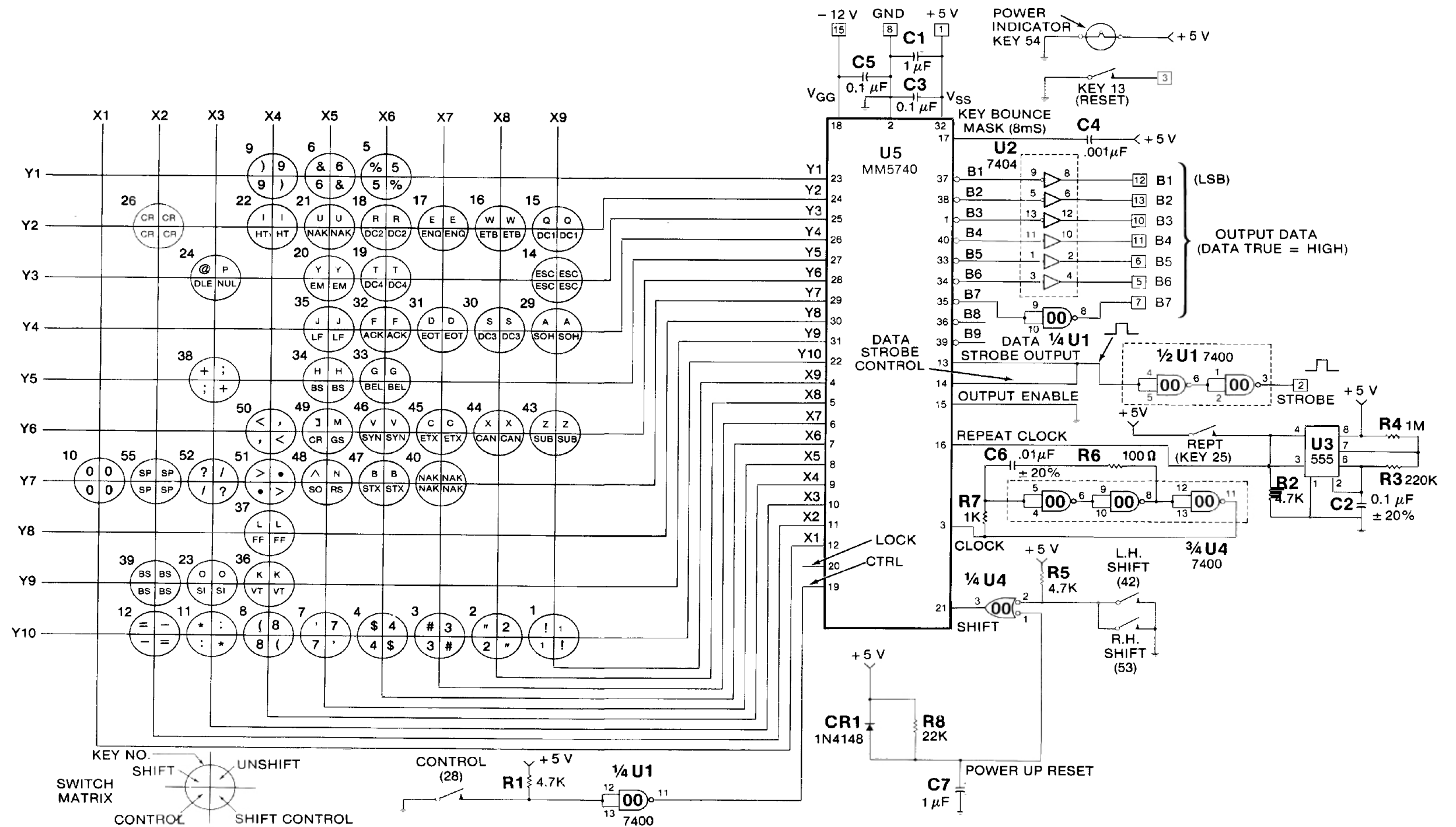
Fig. C-21. Single-piece keyboard.
