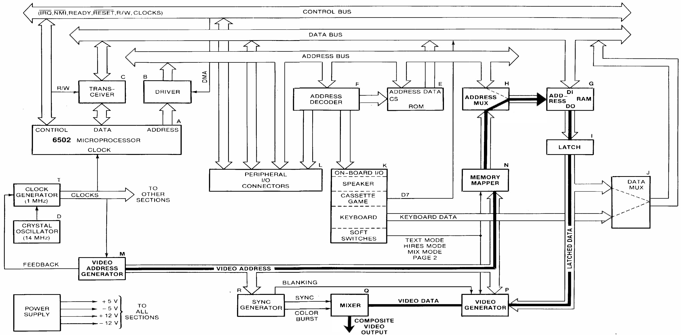
Fig. 2-6. Video-cycle path.
