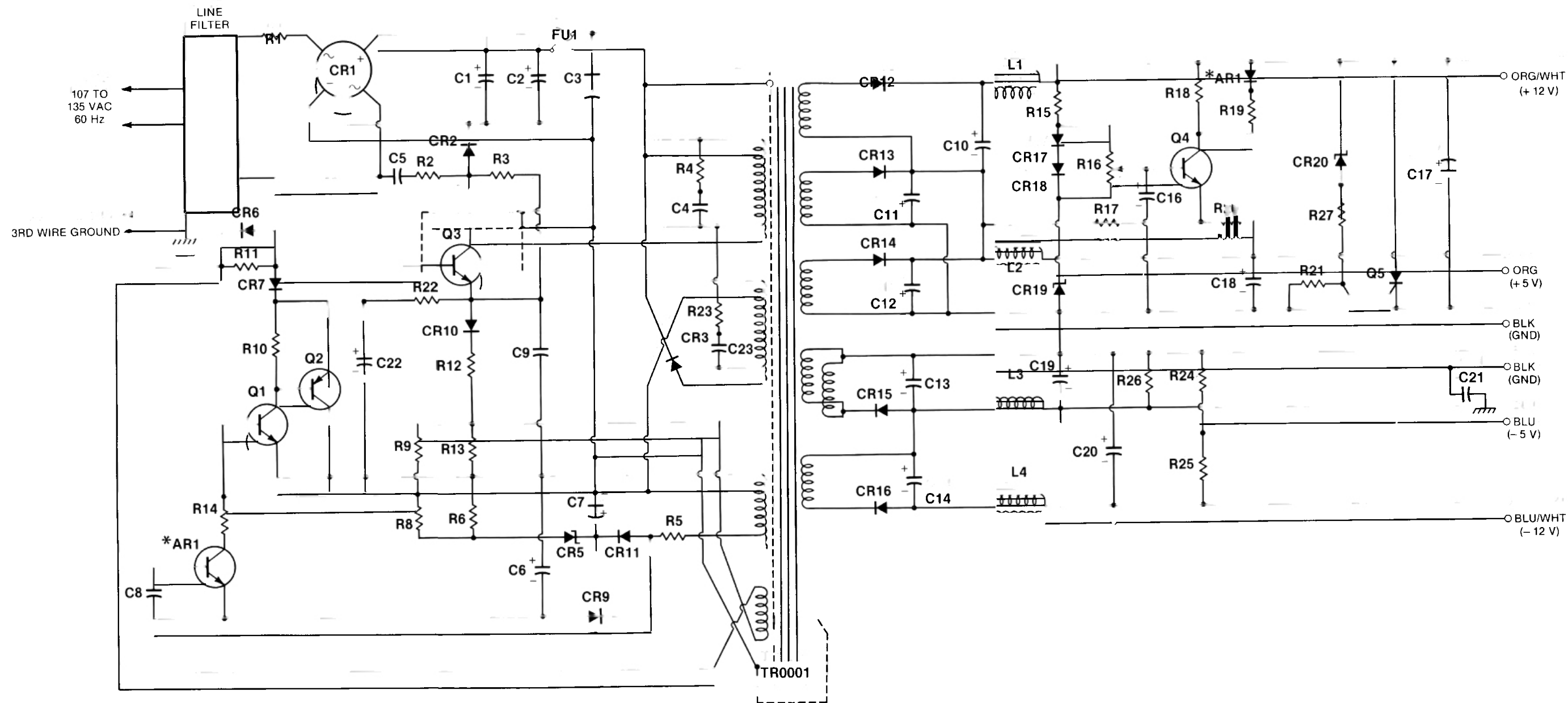
Fig. C-23. Power supply.
