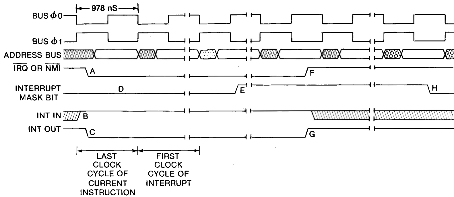
Fig. 6-14. 6502 interrupts.
