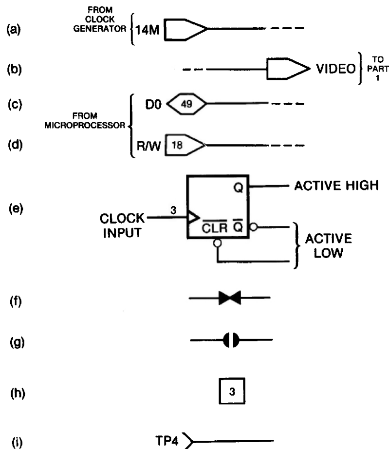
Fig. C-1. Schematic symbols.
