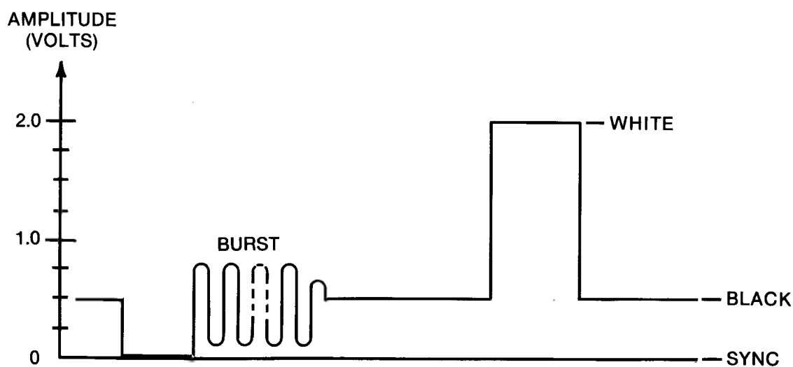
APPLE II COMPOSITE VIDEO OUTPUT MEASURED OPEN CIRCUIT WITH R11 AT MAXIMUM.
