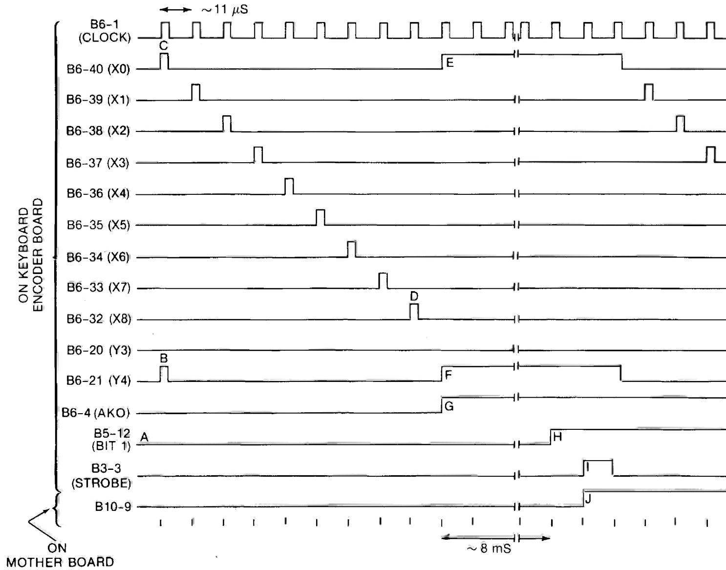
Fig. 7-2. X scan (two-piece keyboard).
