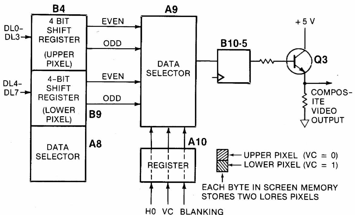
Fig. 8-15. Block diagram of LORES generator.
