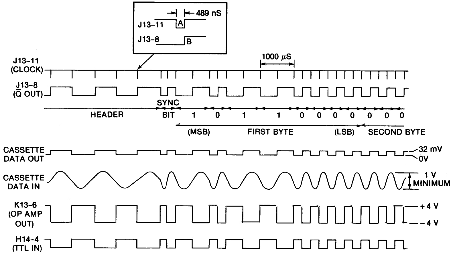
Fig. 7-8. Tape cassette waveforms.
