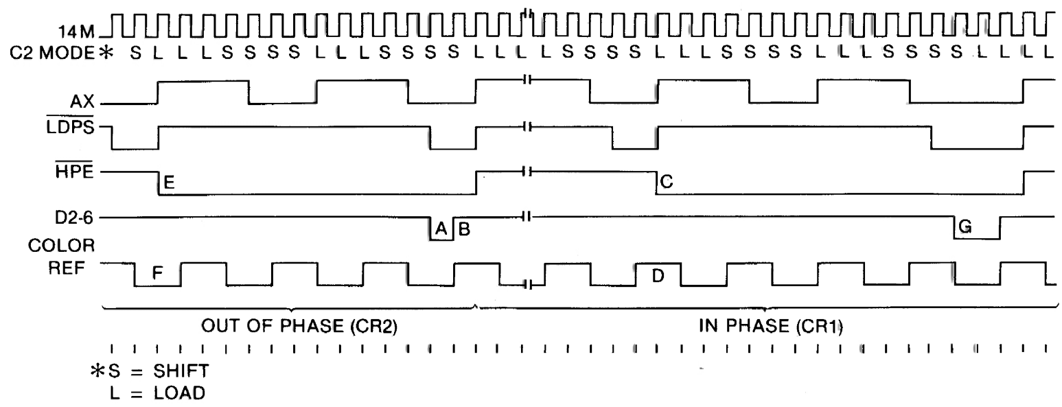
Fig. 3-6. Clock synchronization—CR2.
