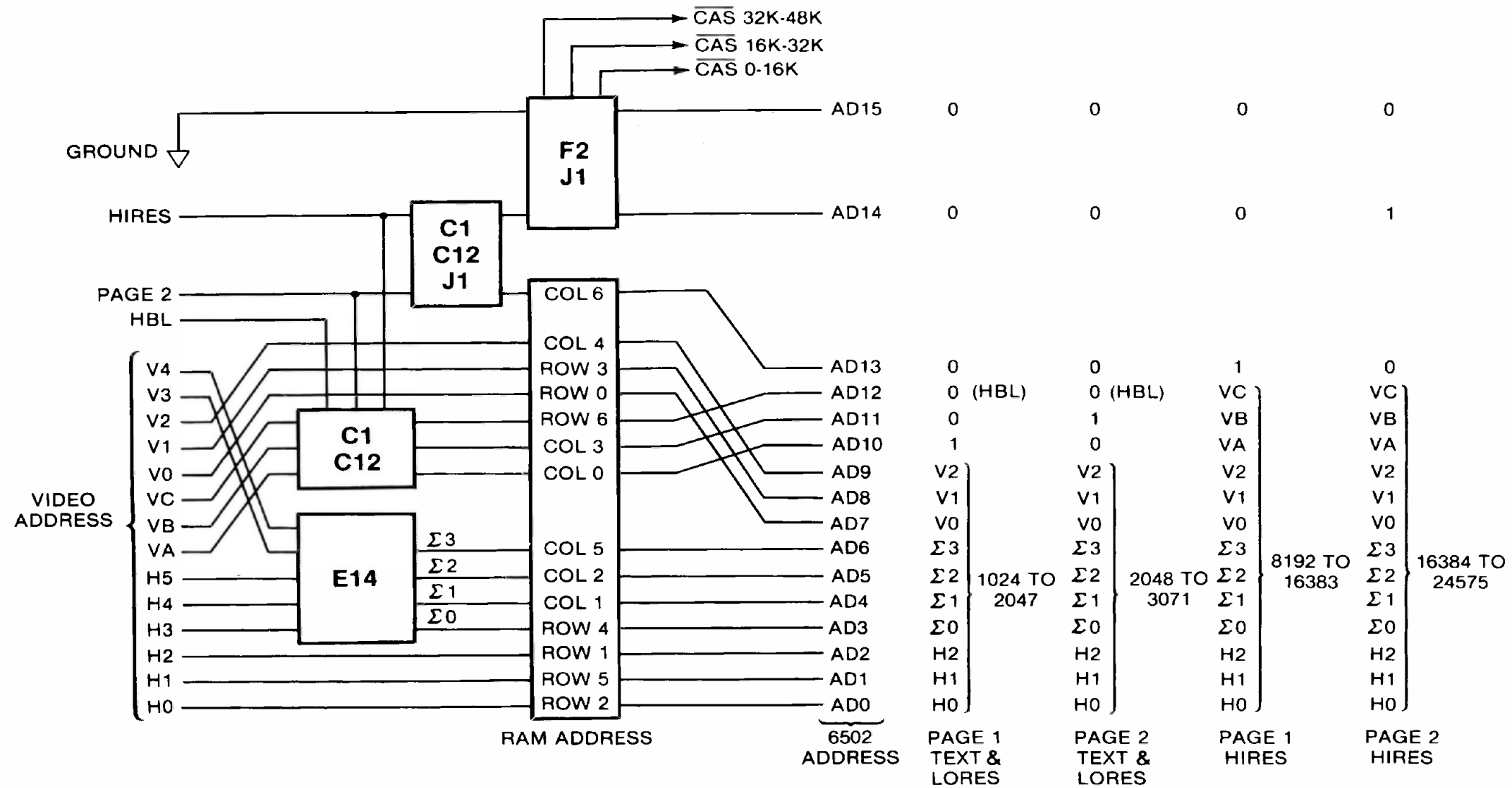
Fig. 5-7. Video mapping.
