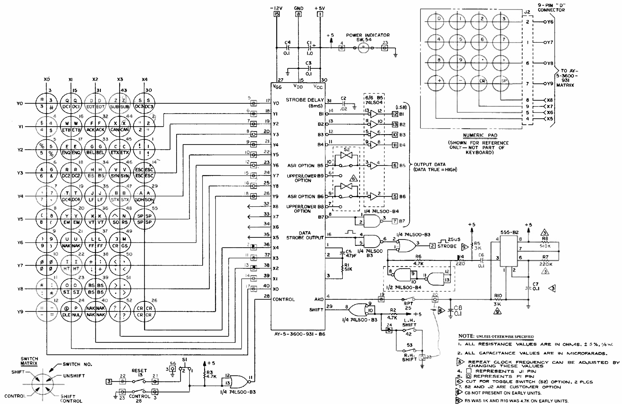
Fig. C-22. Two-piece keyboard.
