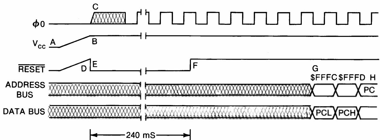
Fig. 6-15. 6502 reset sequence.
