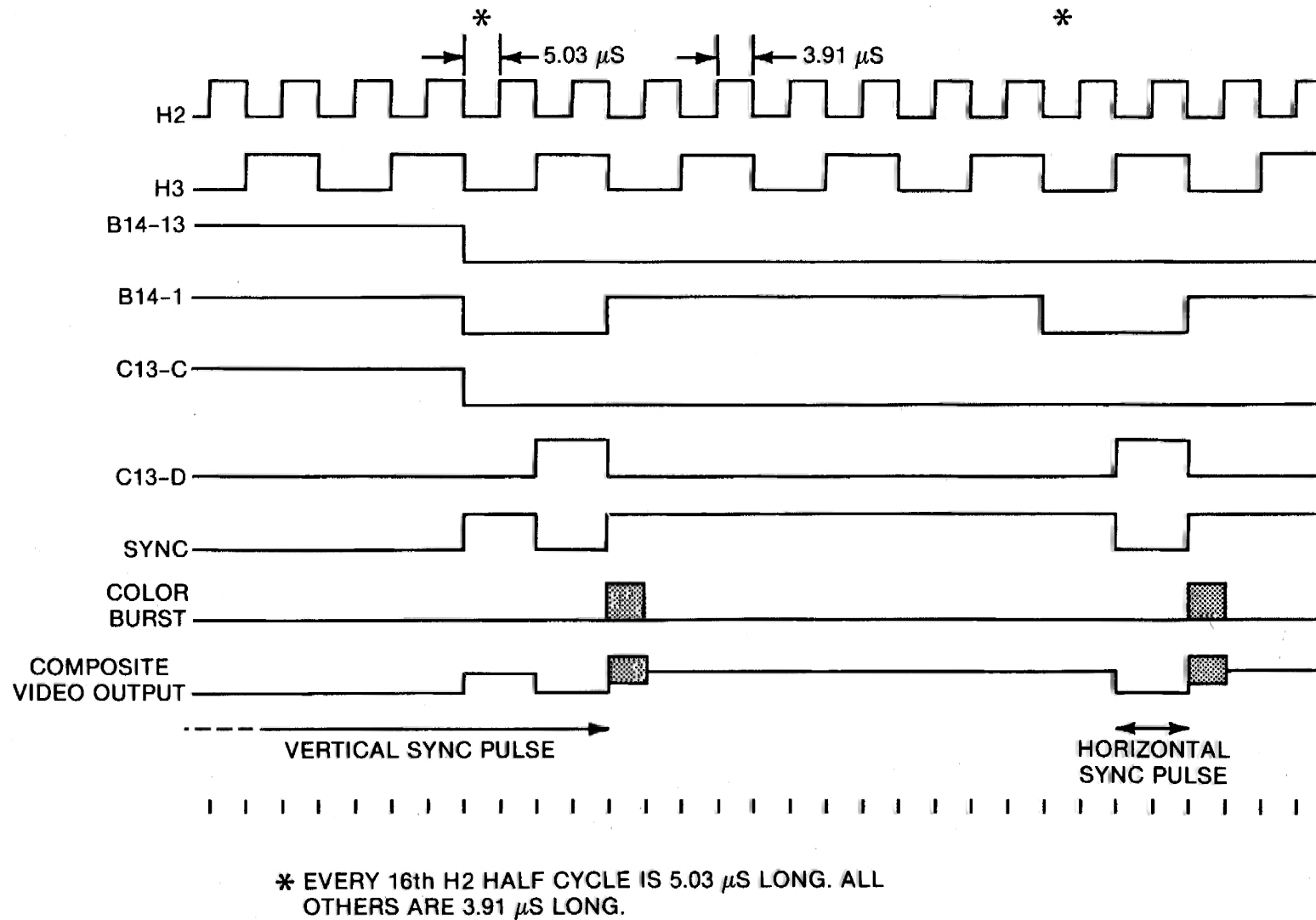
Fig. B-3. Vertical and horizontal sync—Rev. 1.
