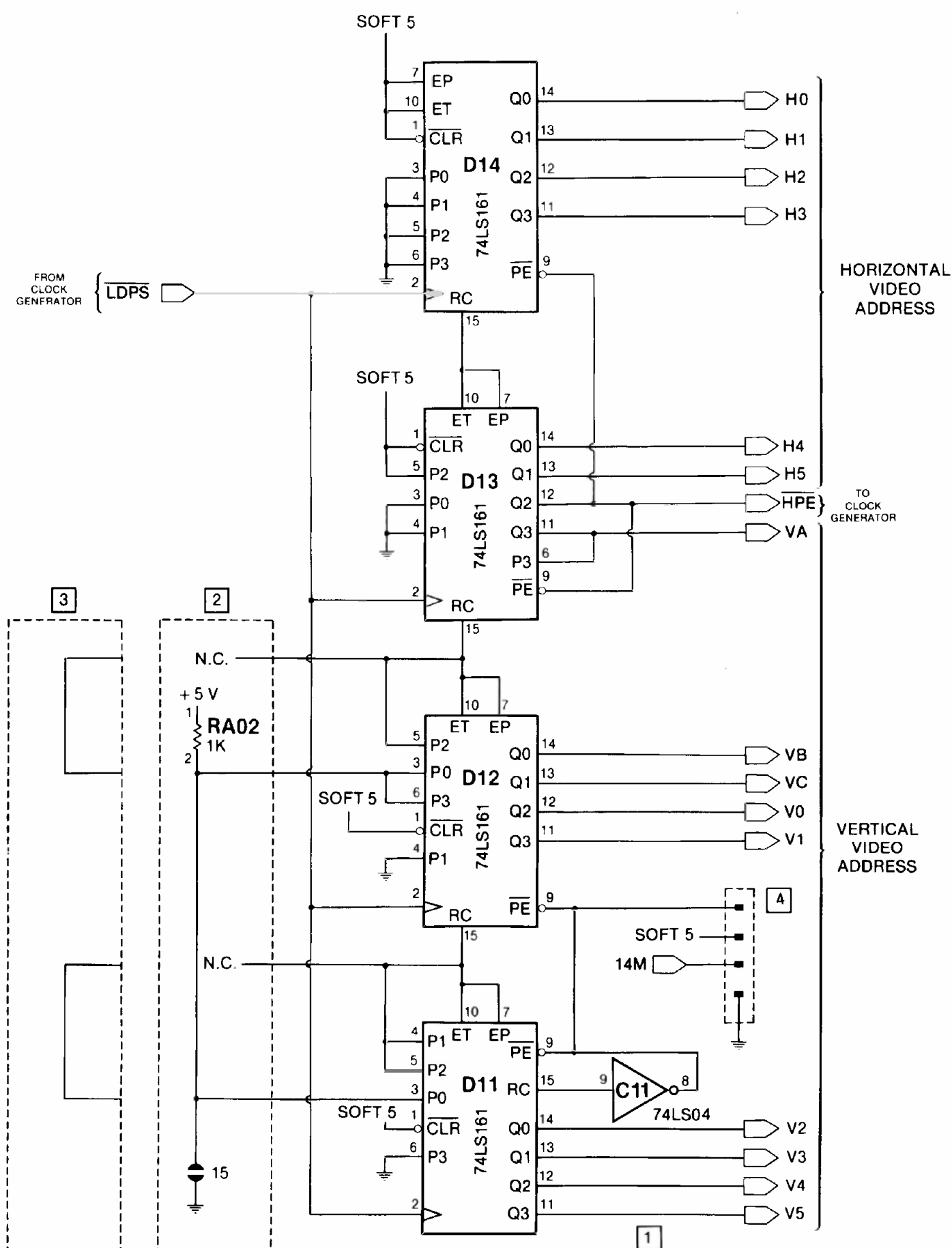
Fig. C-3. Video address generator (all revisions).
