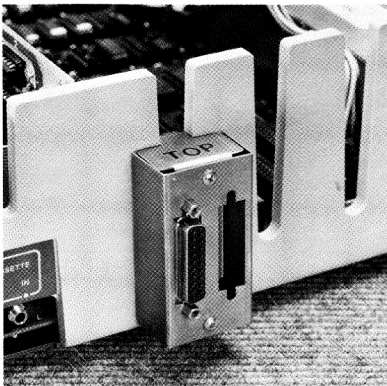
Figure 2-7. Installed Clamp
