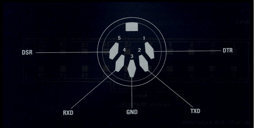
RS 232c-connector Solder side
