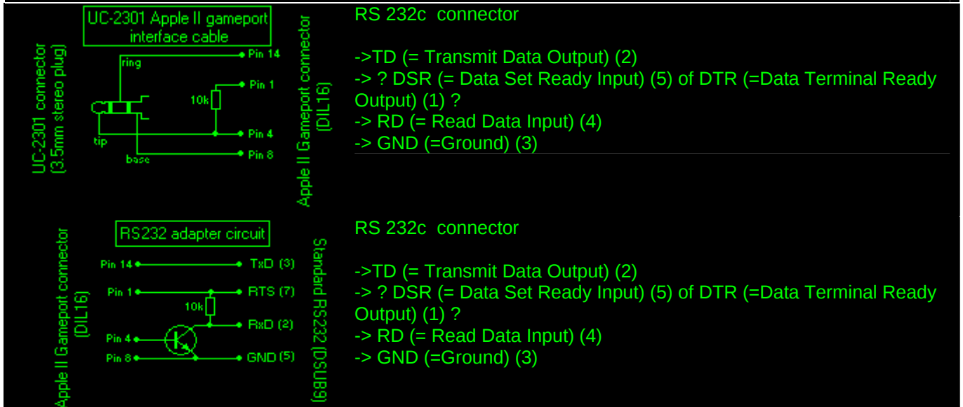
RS 232c-connector Solder side
